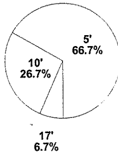
Scoring Range
