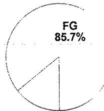
Scoring Distribution
